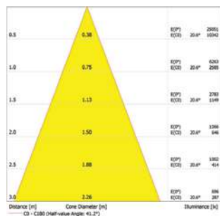
Ø9.5 - 32W - Medium Beam
