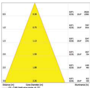
Ø9.5 - 38W - Medium Beam
