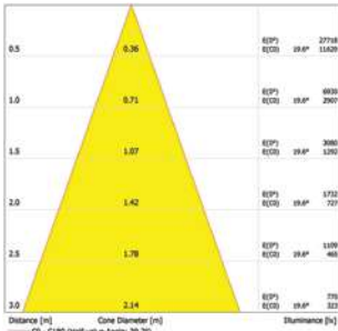
Ø15 -36W - Narrow Beam
