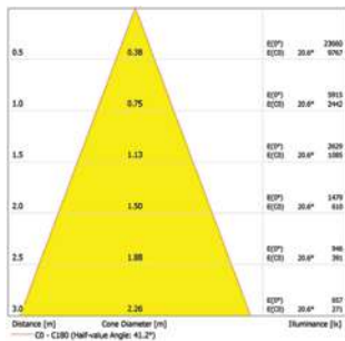
Ø15 - 36W - Medium Beam
