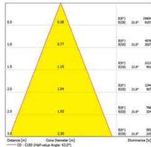
Ø9 - 30W - Medium Beam
