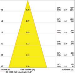
Ø6 -6W - Narrow Beam
