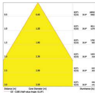
Ø20 - 36W - Medium Beam
