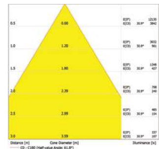
Ø15 - 25W - Medium Beam
