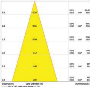
Ø10 -18W - Narrow Beam
