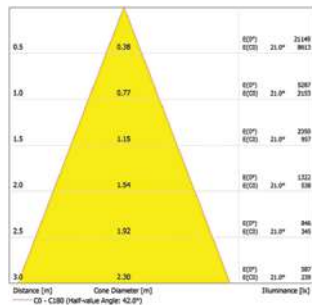
Ø9.5 - 30W - Medium Beam
