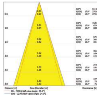
46W - Medium Beam
