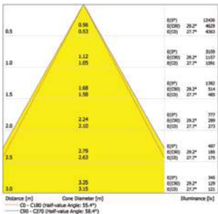
24W - Wide Beam
