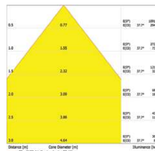
Ø15 - 36W - Medium Beam
