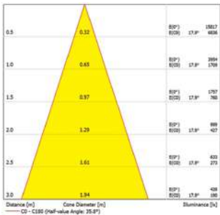
Ø7.5 - 20W - Medium Beam
