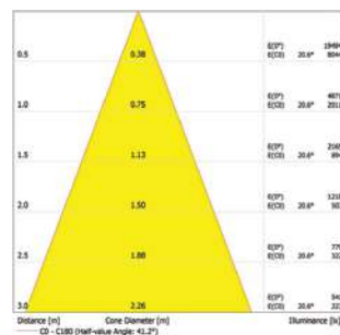
Ø9.5 - 69W - Medium Beam
