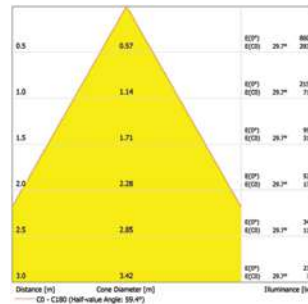
Ø12 - 18W - Medium Beam
