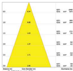
Ø10 - 16W - Narrow Beam
