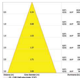
Ø8 - 10W - Narrow Beam
