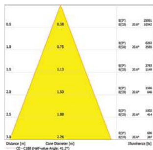
Ø9.5 - 64W - Medium Beam
